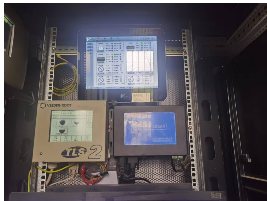
防渗漏检测仪
